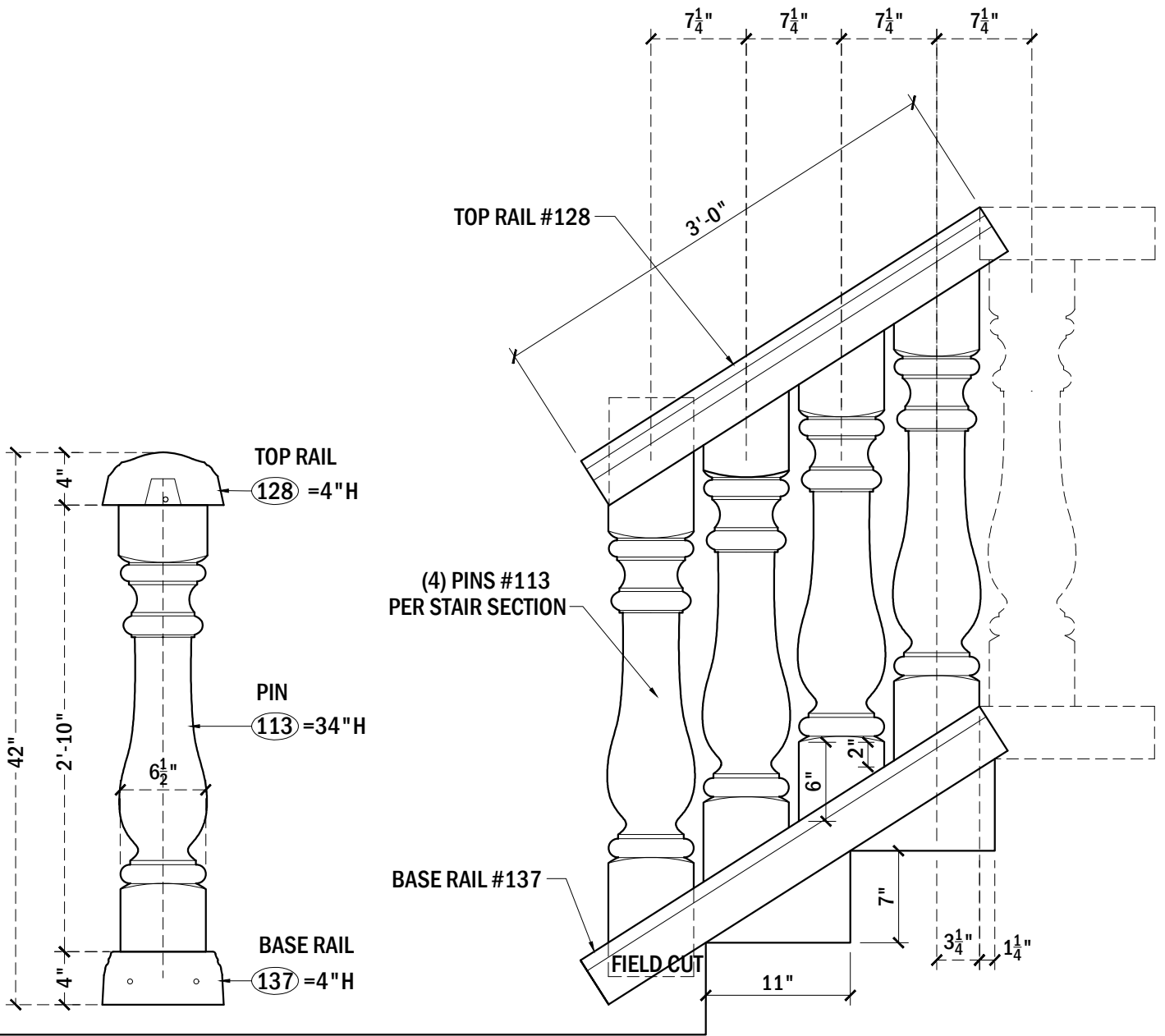
PROFILE VIEW
