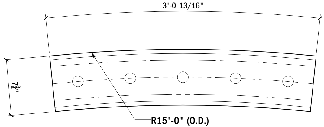
TOP VIEW, BASE RAIL #136
