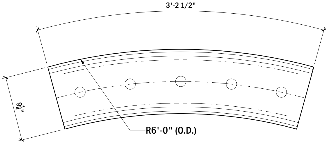
TOP VIEW, BASE RAIL #141
