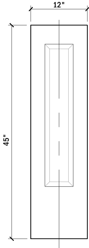
ELEVATION VIEW
