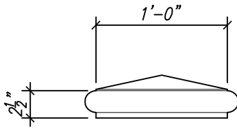
ELEVATION VIEW
