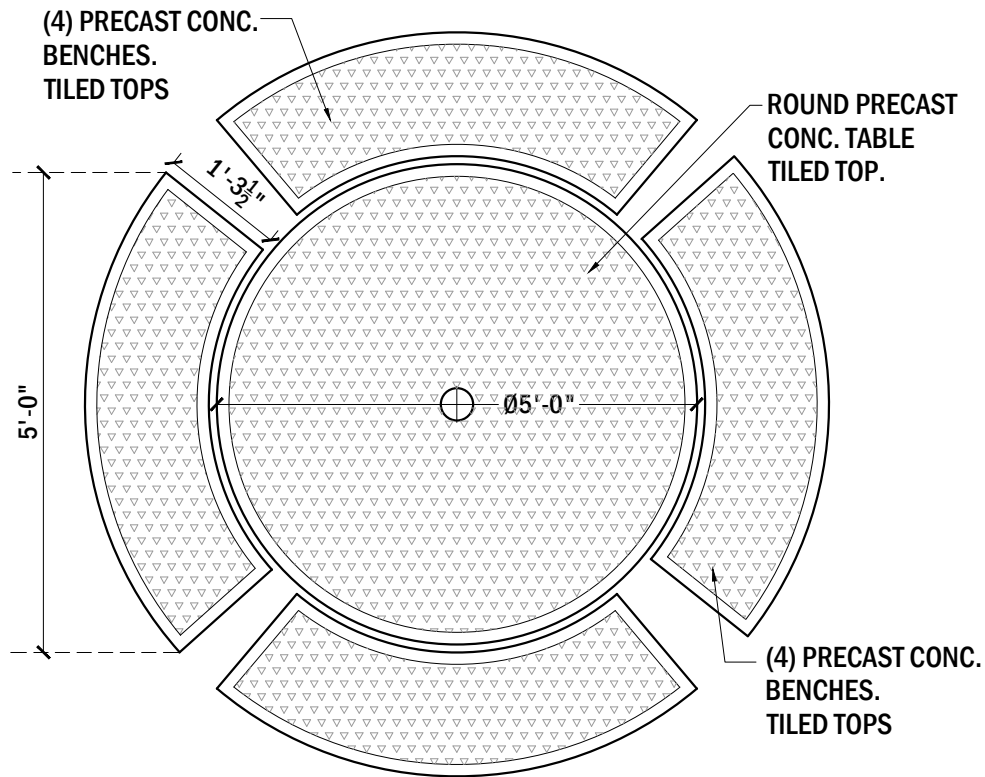
PLAN VIEW, TABLE #614
