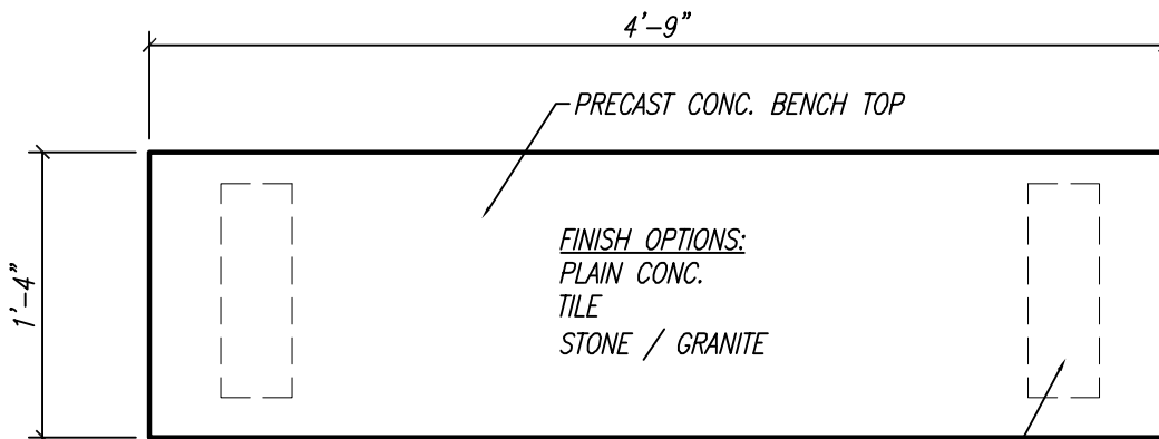
A PLAN VIEW 1" = 1'-0"
