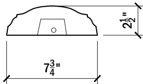
SIDE VIEW TOP RAIL #122
