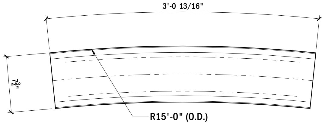
TOP VIEW, TOP RAIL #127
