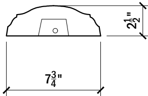
SIDE VIEW TOP RAIL #127
