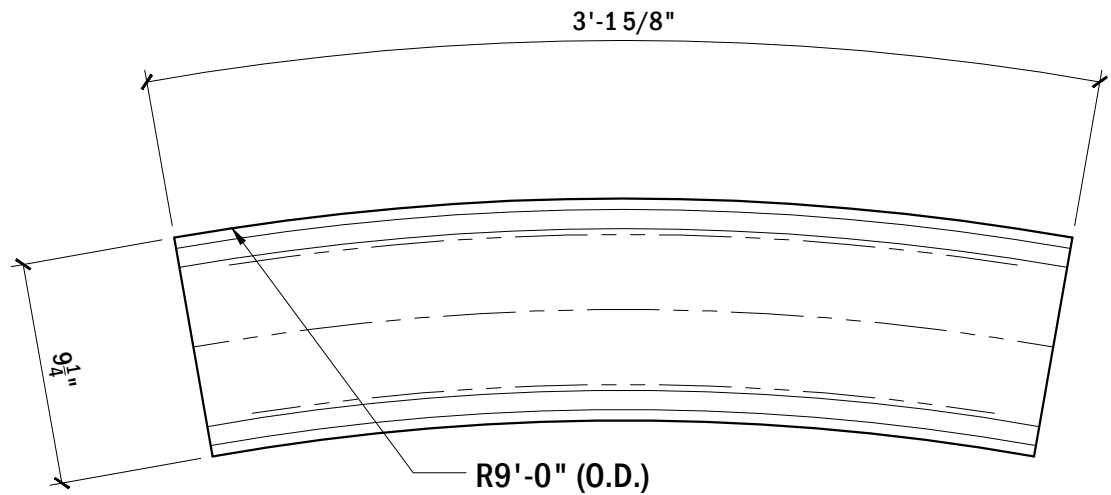
TOP VIEW, TOP RAIL #129
