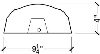
SIDE VIEW TOP RAIL #129
