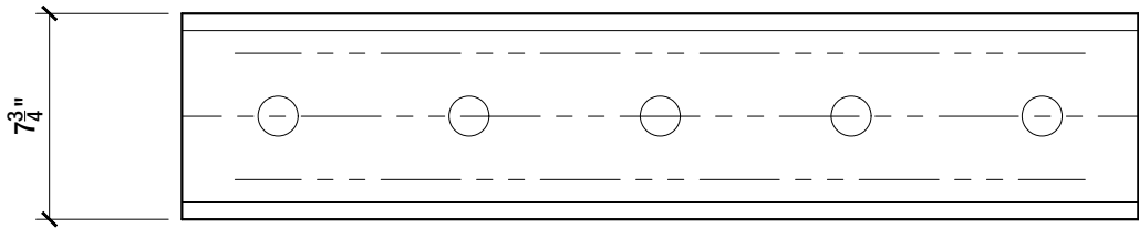
TOP VIEW, BASE RAIL #132
