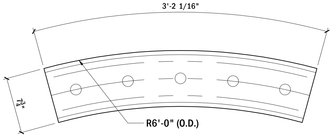
TOP VIEW, BASE RAIL #134
