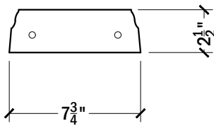
SIDE VIEW BASE RAIL #134
