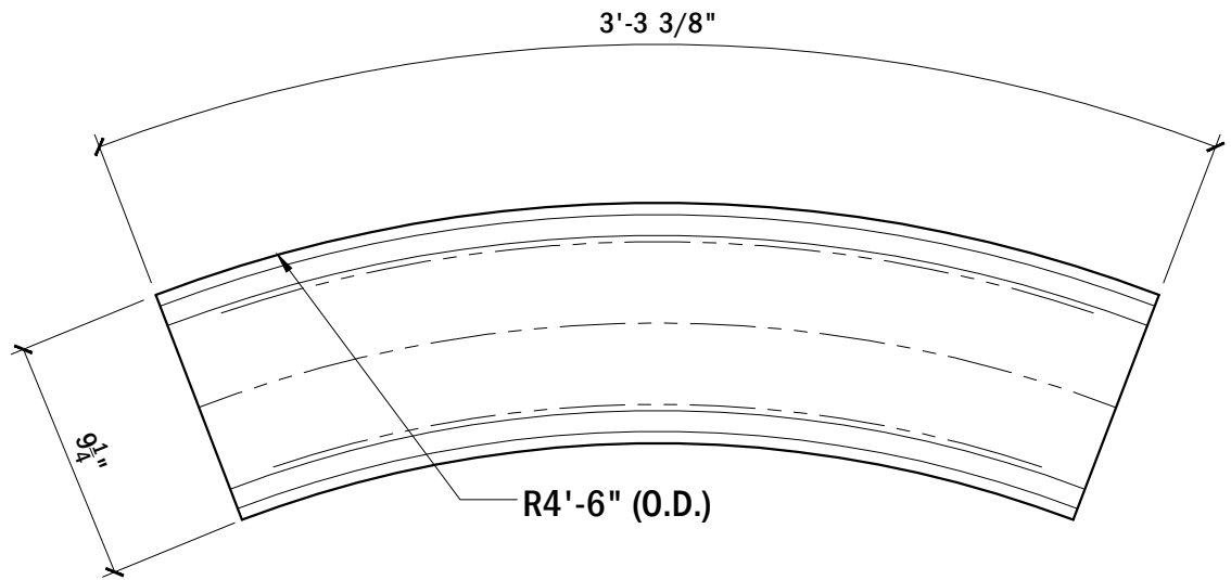
TOP VIEW, TOP RAIL #142
