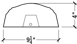
SIDE VIEW TOP RAIL #142
