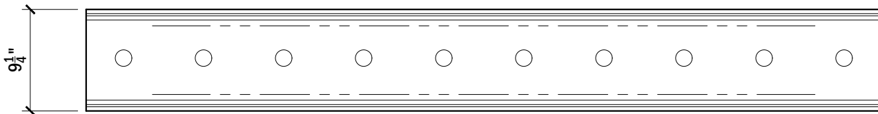
TOP VIEW, BASE RAIL # 146
