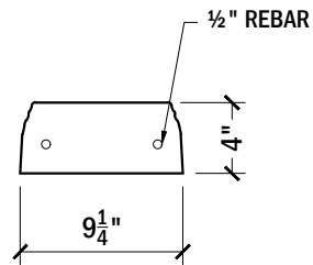
SIDE VIEW, BASE RAIL # 146
