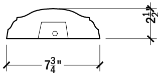
SIDE VIEW TOP RAIL #160
