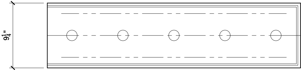
TOP VIEW, BASE RAIL #163
