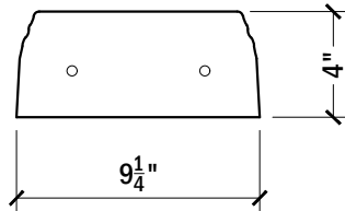
SIDE VIEW BASE RAIL #163
