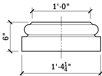
ELEVATION VIEW
