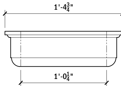
ELEVATION VIEW
