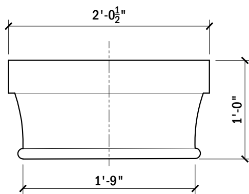
ELEVATION VIEW
