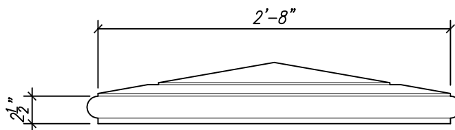
ELEVATION VIEW
